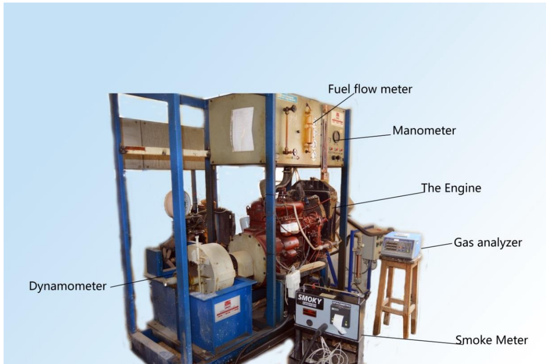
Figure (1) photograph of the engine
