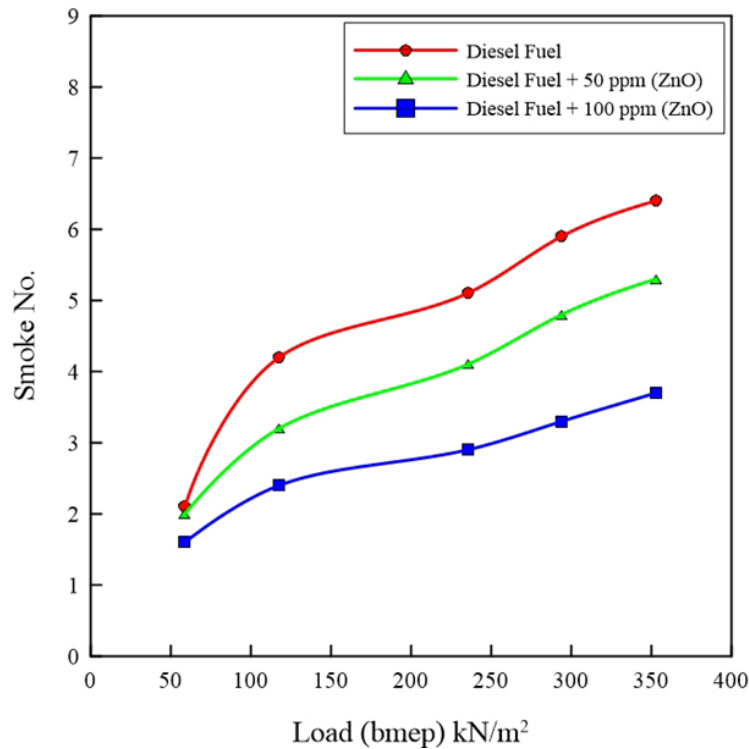
Figure (5) the smoke number for the three types of fuels at different loads.
