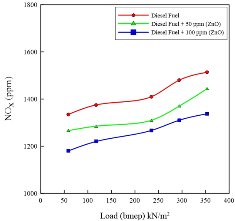
Figure (4) nitrogen oxide NO x emissions for the three types of fuels at different loads.
