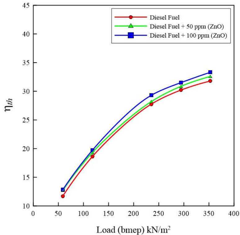
Figure (3) The Brake Thermal efficiency at different loads for three types of fuels.
