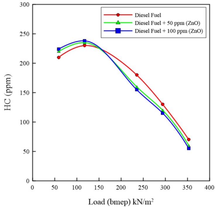
Figure (6) the unburned hydrocarbon emissions for the three types of fuels at different loads.
