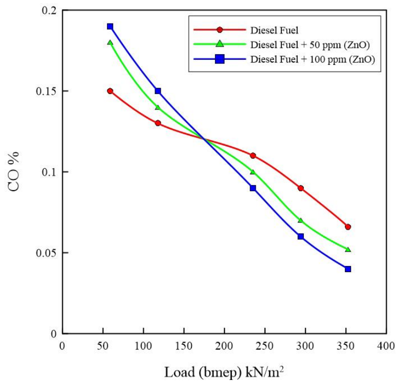
Figure (5) the carbon monoxide emissions for the three types of fuels at different loads.
