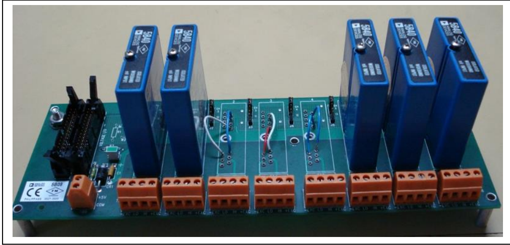
Fig. 3. The GPIB card with thermocouple modules.
