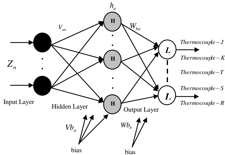
DFig. 5. The multi-layer perceptron neural networks act as cognitive linearization model.
