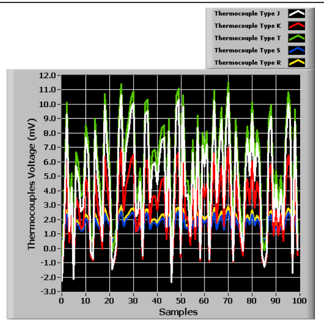
Fig. 8. Testing set thermocouple voltage.
