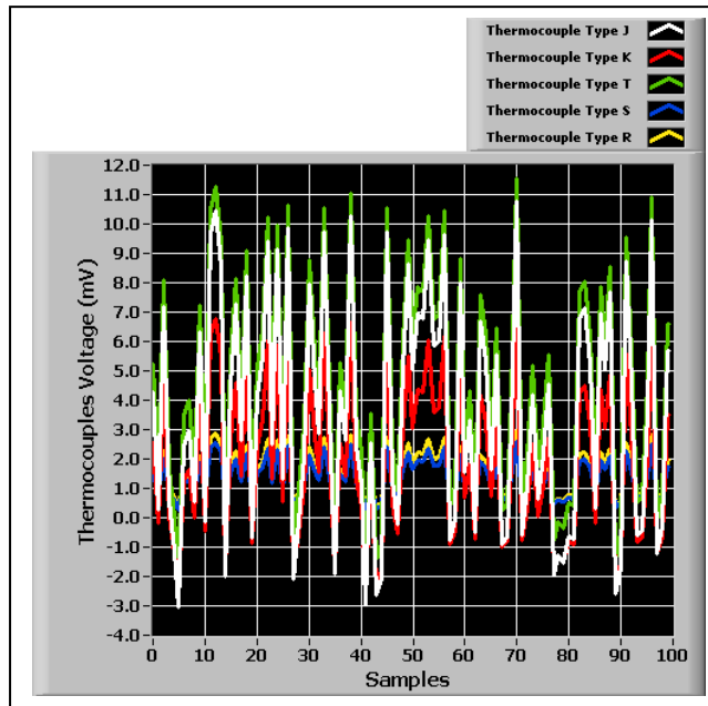
Fig. 7. Learning set thermocouple voltage.
