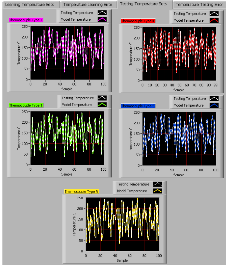
Fig. 11. Model temperature output for testing set thermocouple voltage.
