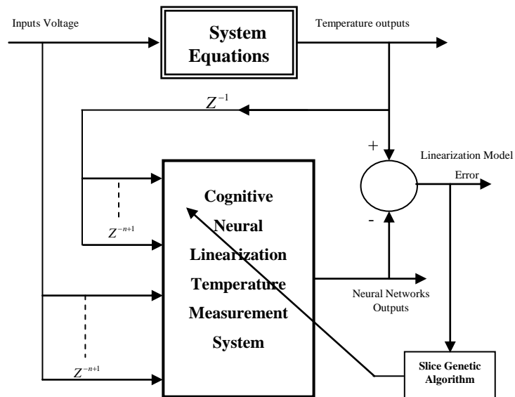
Fig. 6. The series-parallel structure model.
