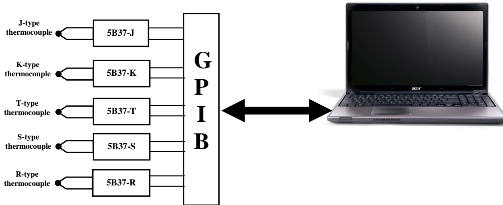
Fig. 1. Temperature measurement system.
