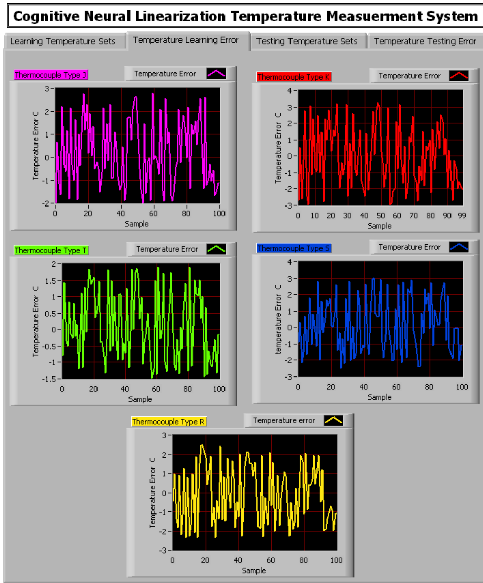
Fig. 10. Temperature model error for learning set thermocouple voltage.
