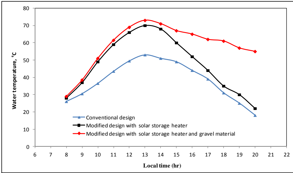
Fig. 8. The hourly temperature variation for the modified and conventional solar still.
