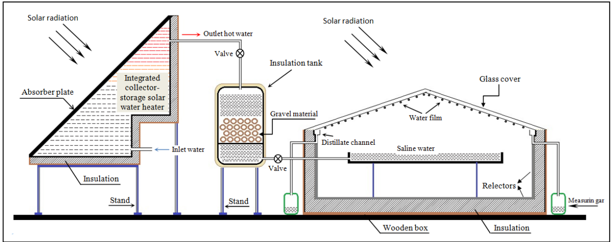
Fig.2. Schematic diagram of the experimental setup for the modified solar still.
